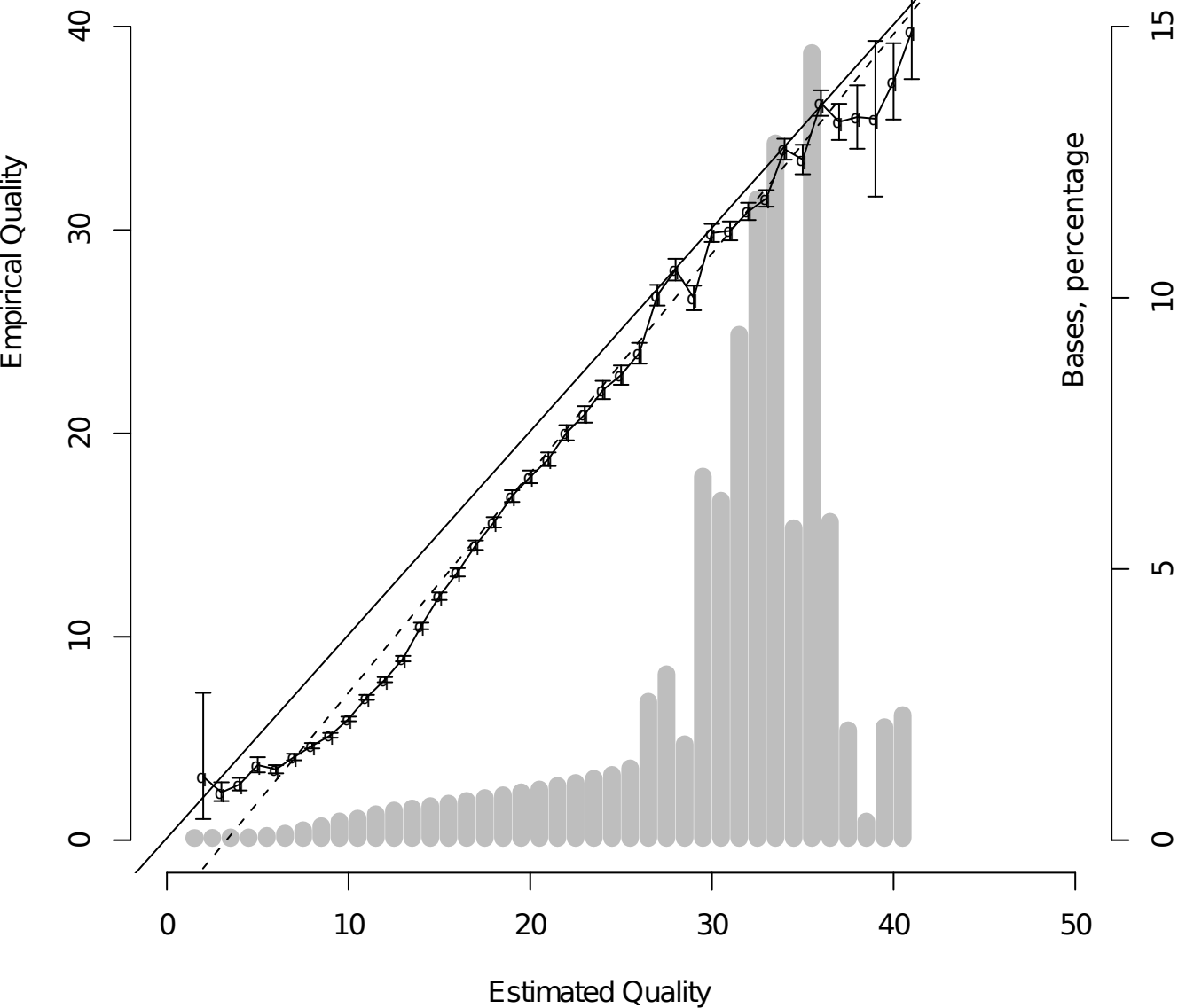
AYB, calibrated on \phi X174 L2
