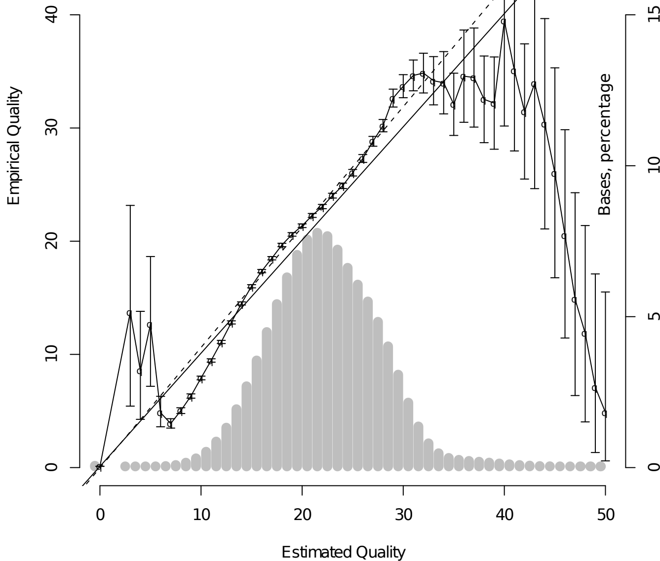
Ibis, trained on Ibis Test
